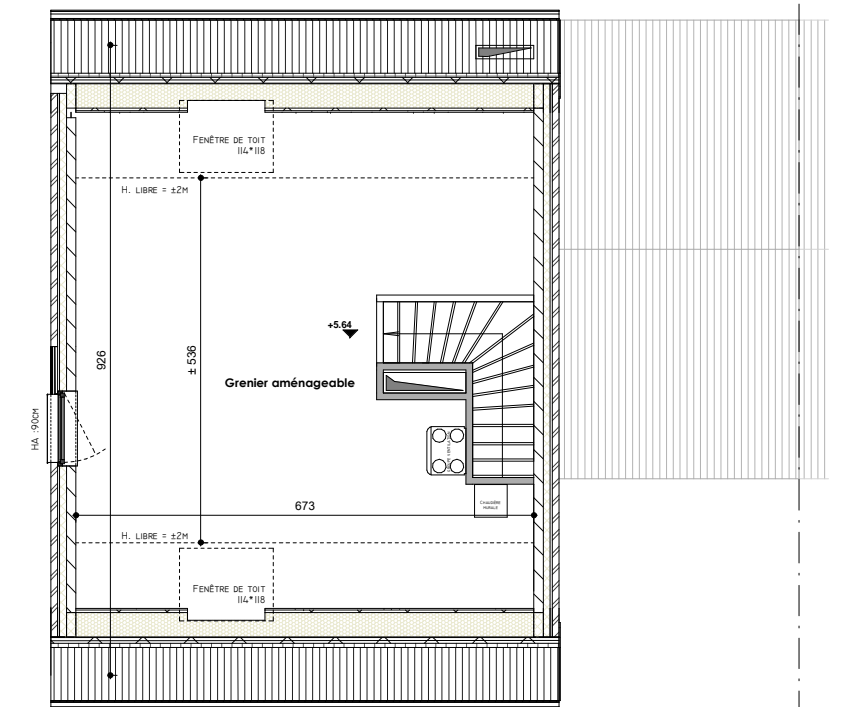
Combles
